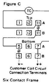
480 Volts – Two Coil Cutoff Contacts Wired in Circuit
