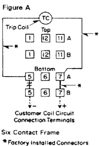
Wiring Diagrams – 24 Thru 250 Volts
