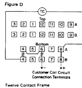
480 Volts – Two Coil Cutoff Contacts Wired in Circuit
